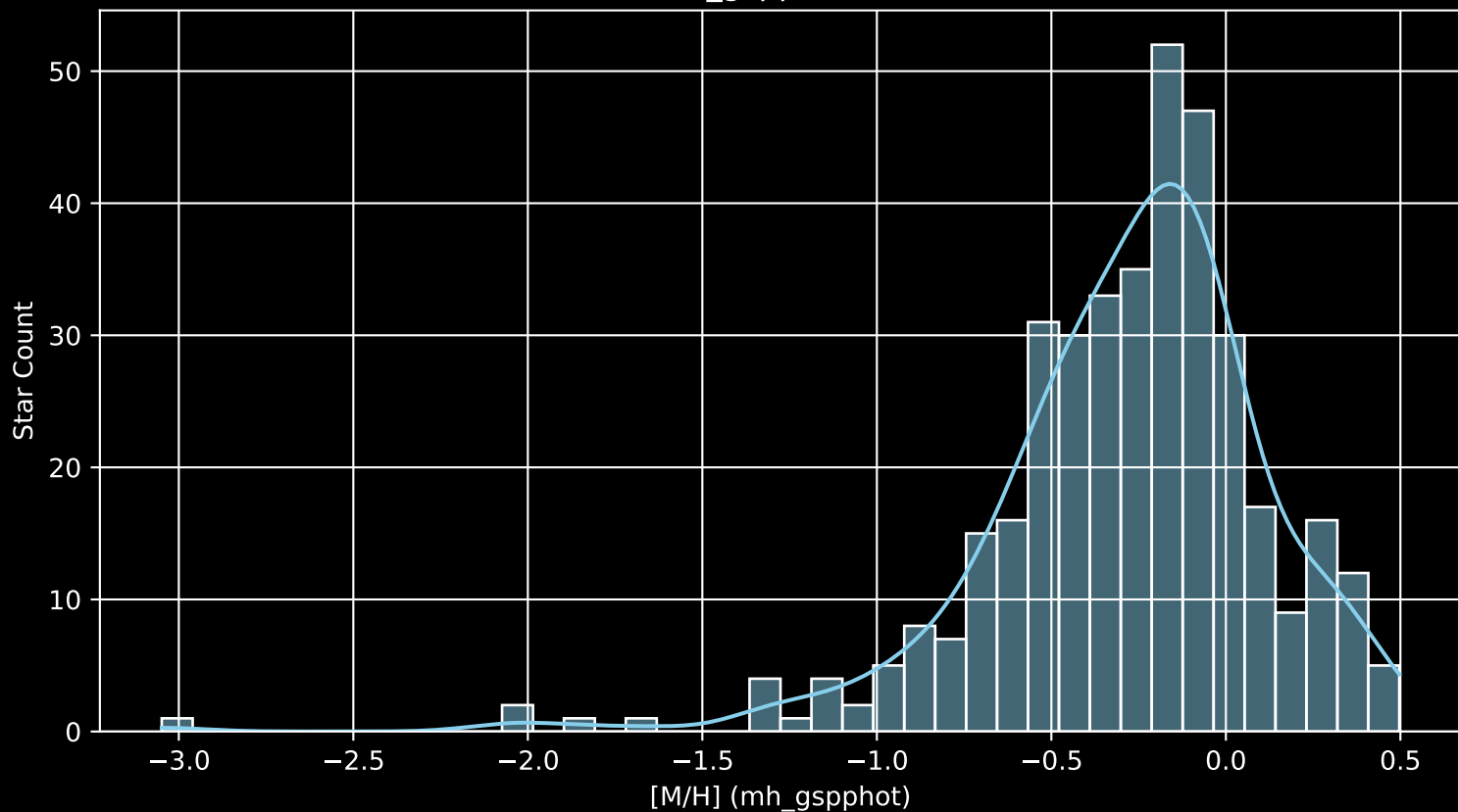
APOGEE DR17 Field: [ORPHAN-5 [M/H] (mh_gspphot) (n= 384)
