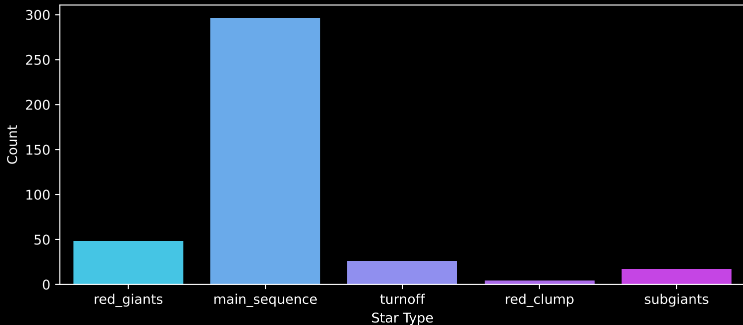
APOGEE DR17 Field: [ORPHAN-5] Count plot of Star Type
