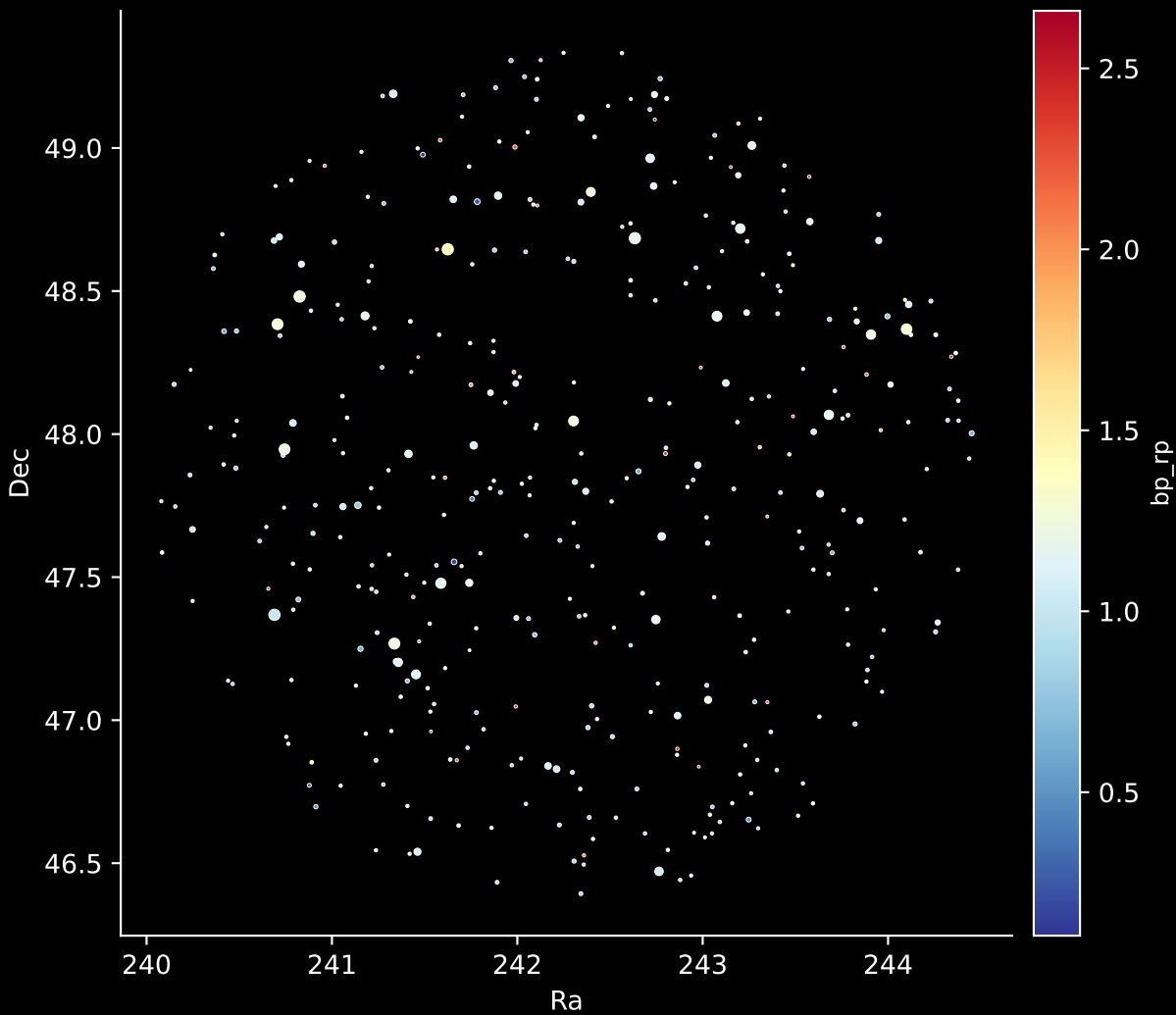
APOGEE DR17 Field: [ORPHAN-5] Stars: 391
