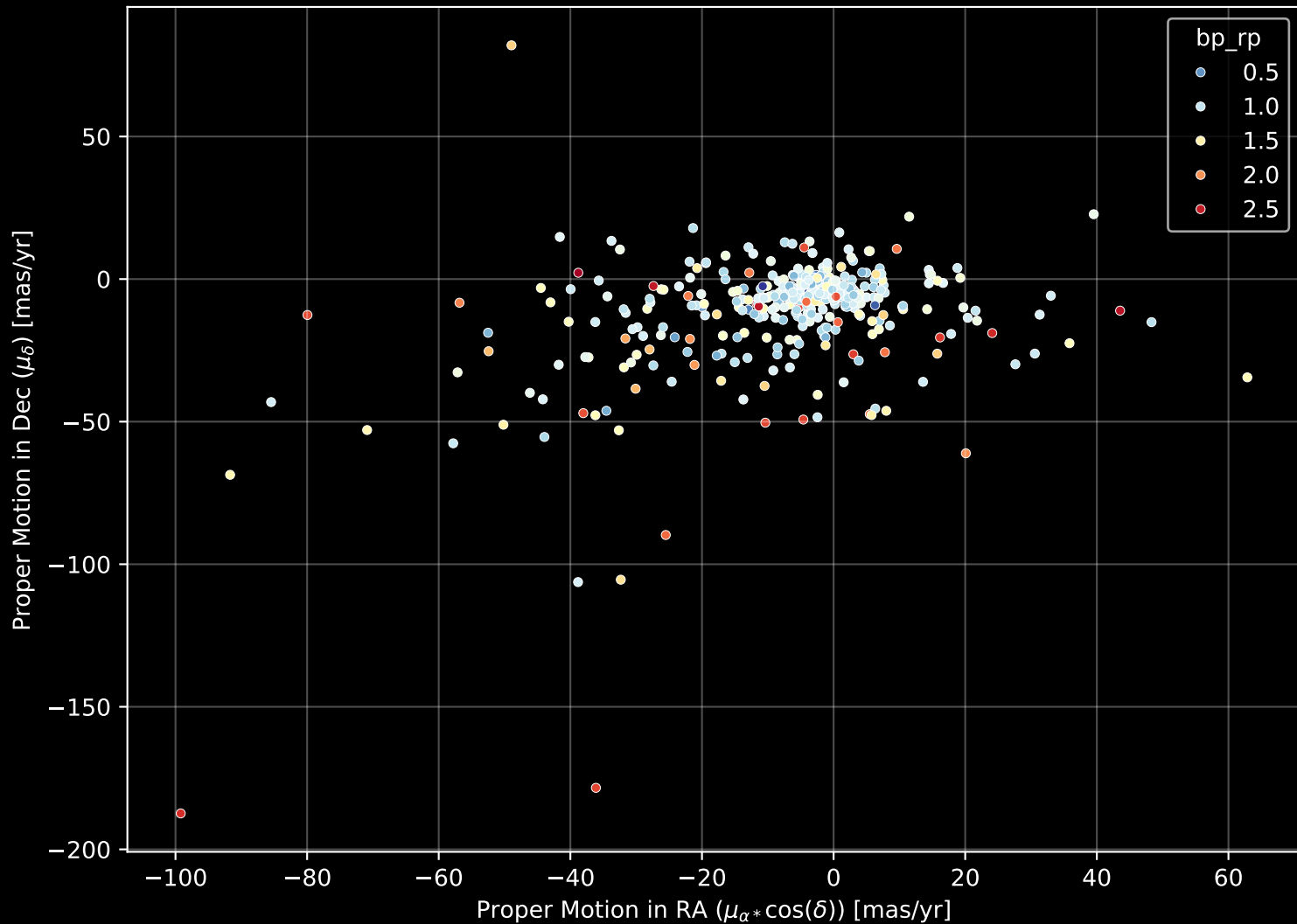
APOGEE DR17 Field: [ORPHAN-5] Proper Motion Diagram (n= 391)
