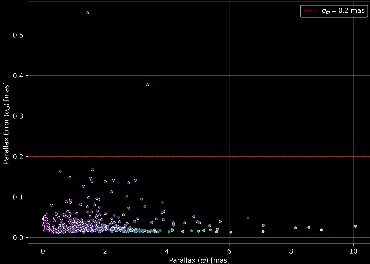
APOGEE DR17 Field: [ORPHAN-5] Parallax Quality (n= 391)
