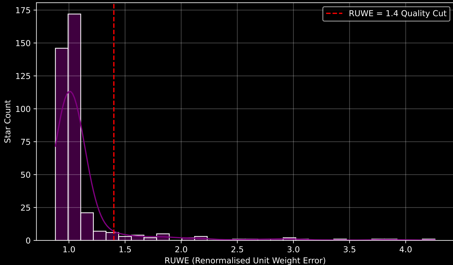
GAPOGEE DR17 Field [ORPHAN-5] RUWE Distribution (n= 381)
