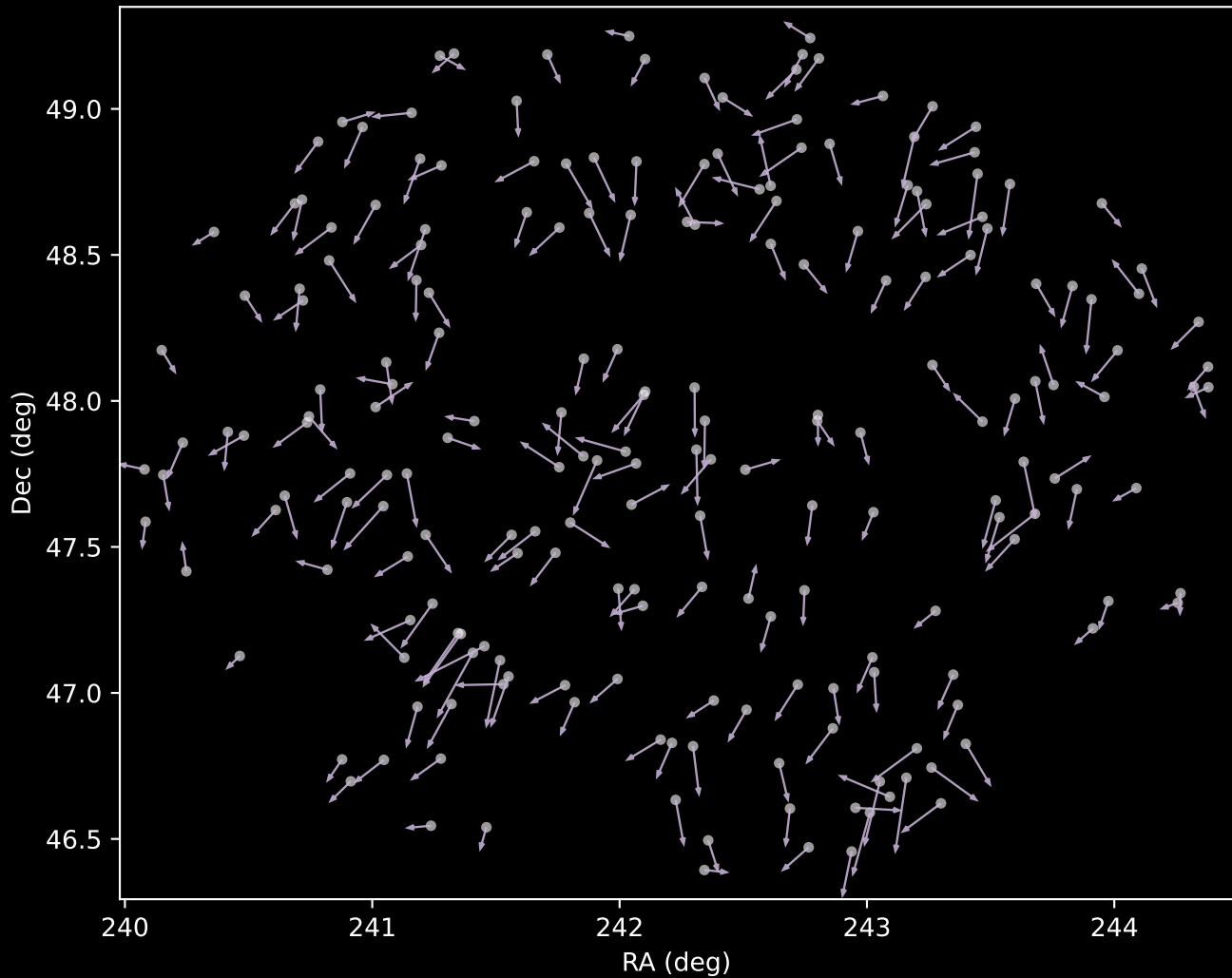
APOGEE DR17 Cluster 9 Proper Motion Vectors (n=208)
